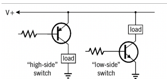
(a) Low Side vs High Side Switching
